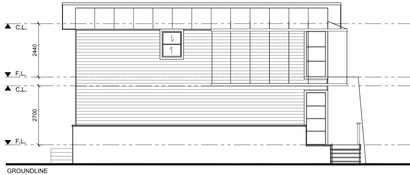
ELEVATION C
